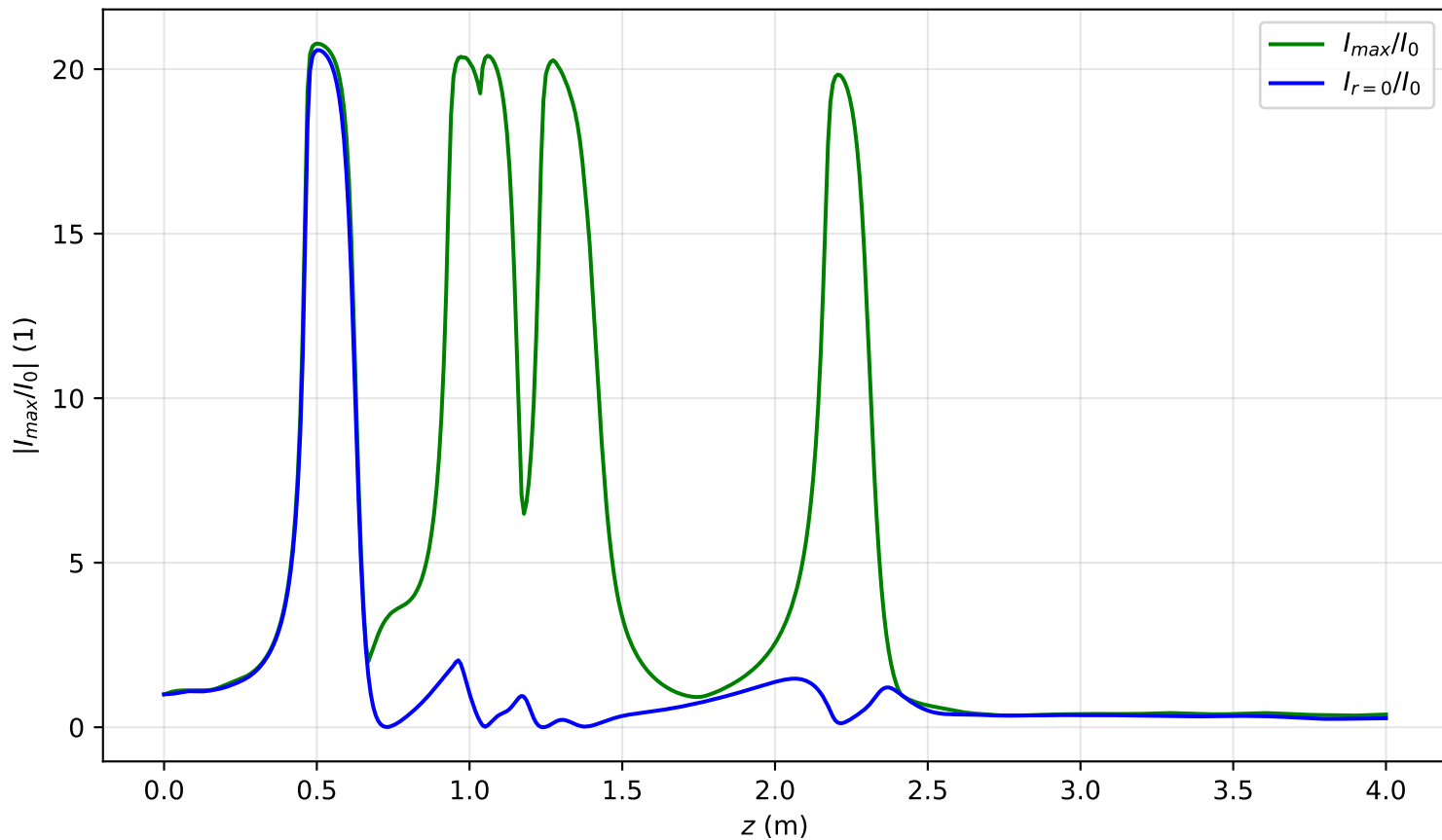
I_{max}(x=0, y=0, z)/I_0 , Pin=5.3Pcr, noisy input, artificial time
